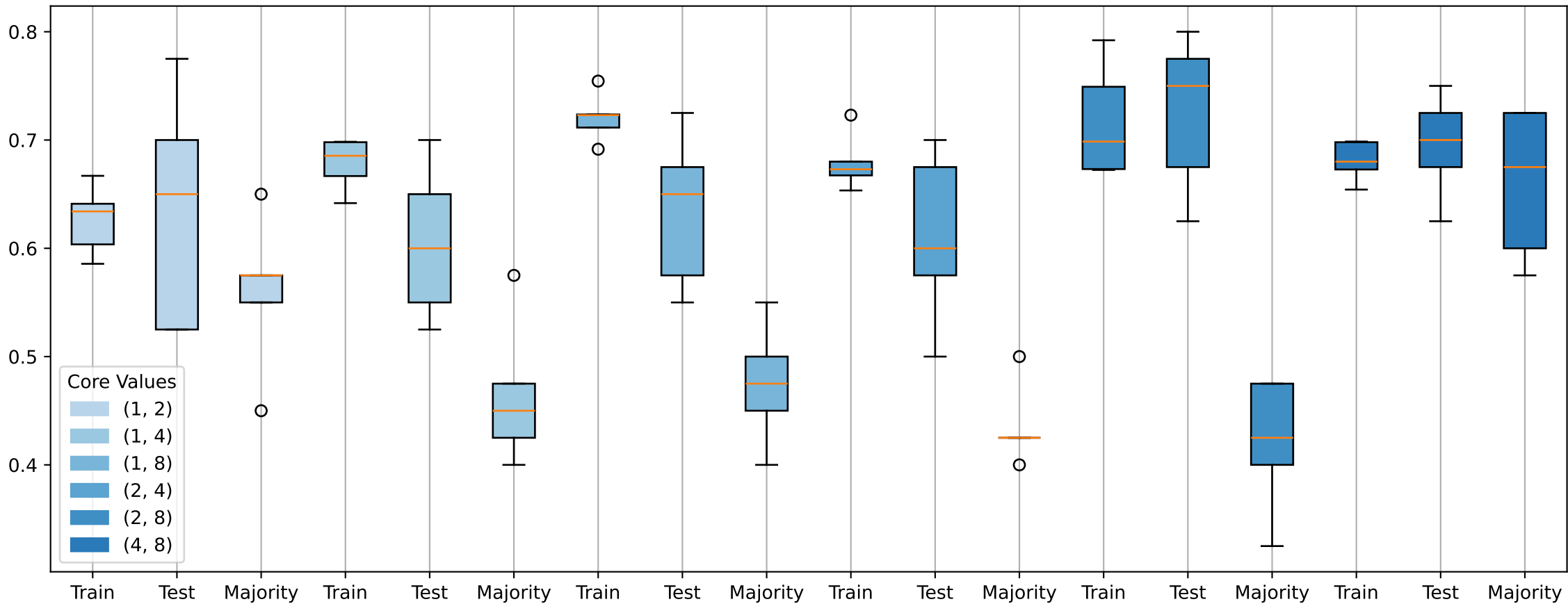
Cplex Scores
