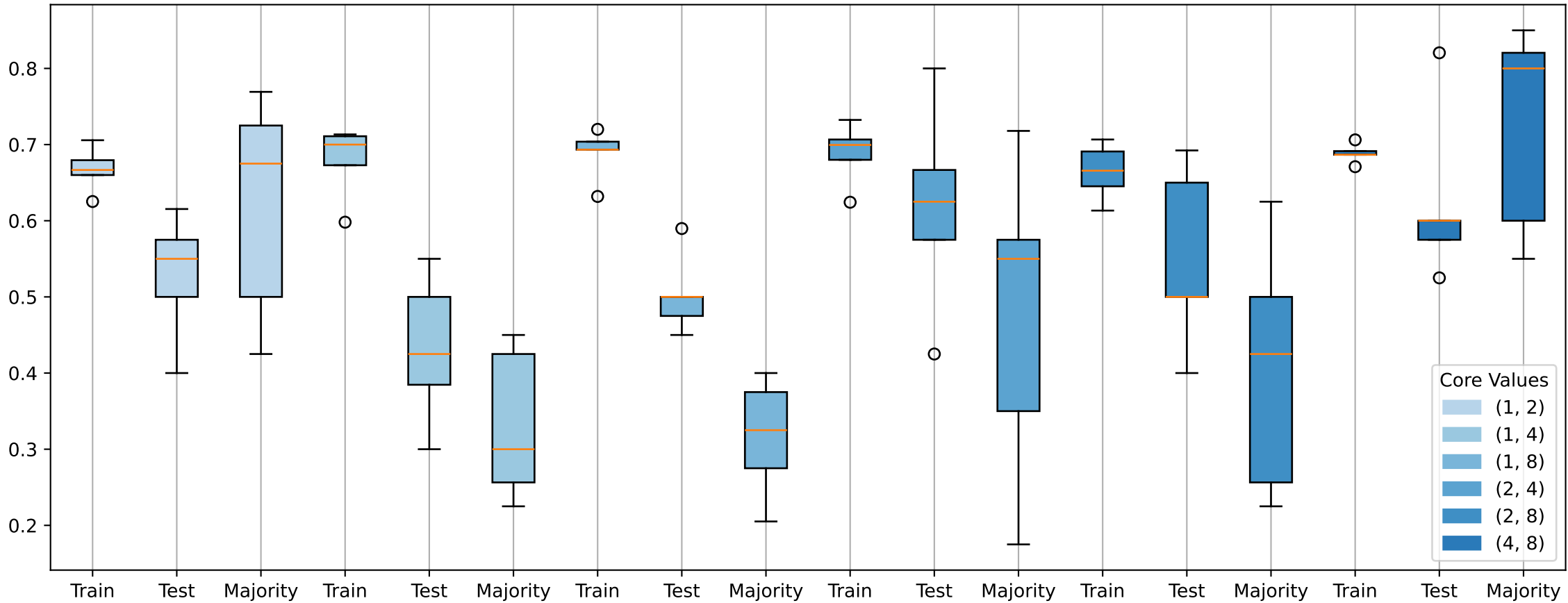
Gecode Scores
