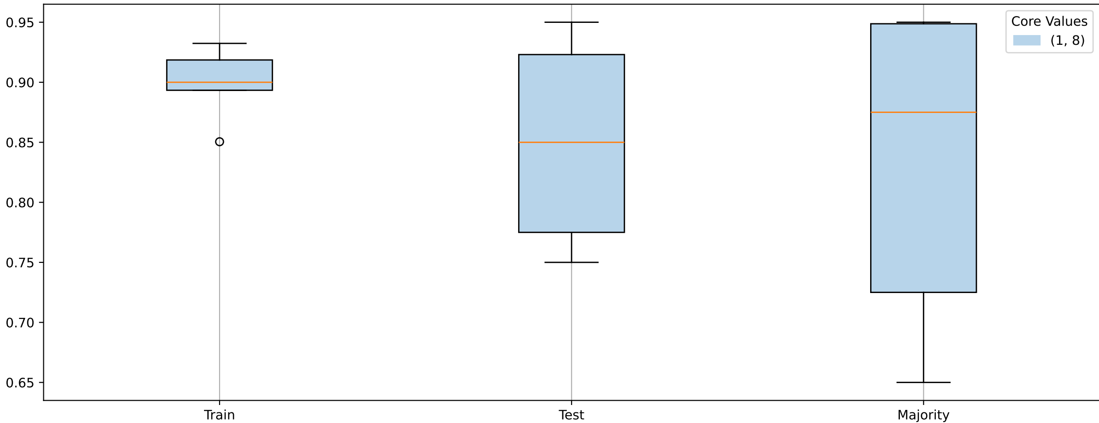
Or-tools Scores
