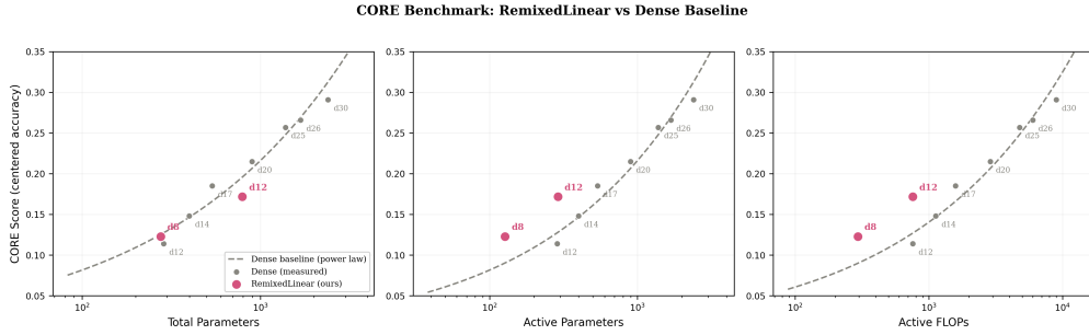
Figure 3: CORE score vs. model size and compute. Left: Total parameters — Remix falls on the dense curve, reflecting K \times storage. Middle/Right: Active parameters and active FLOPs — Remix achieves 34–36% higher CORE scores at matched compute, confirming the scaling improvement is not a parameter-counting artifact.
