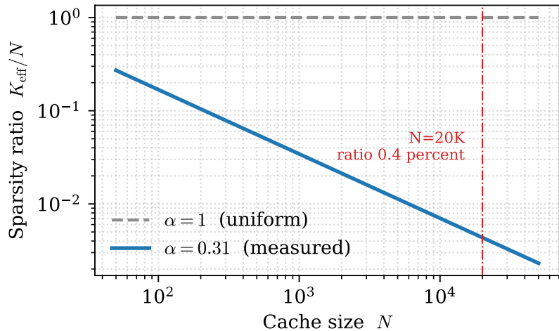
(b) Effective sparsity \sim N^{\alpha-1}
