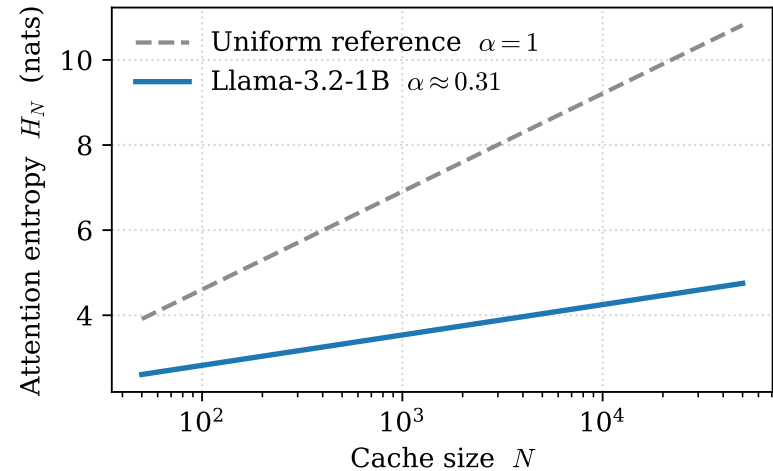
(a) H_N = \alpha \log N + \beta , \alpha < 1
