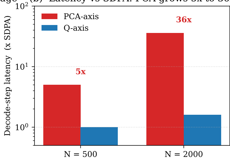
(b) Latency vs SDPA: PCA grows 5x to 36x
