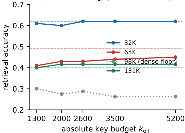
Sparse acc vs k_{\text{eff}} (dashed = dense)
