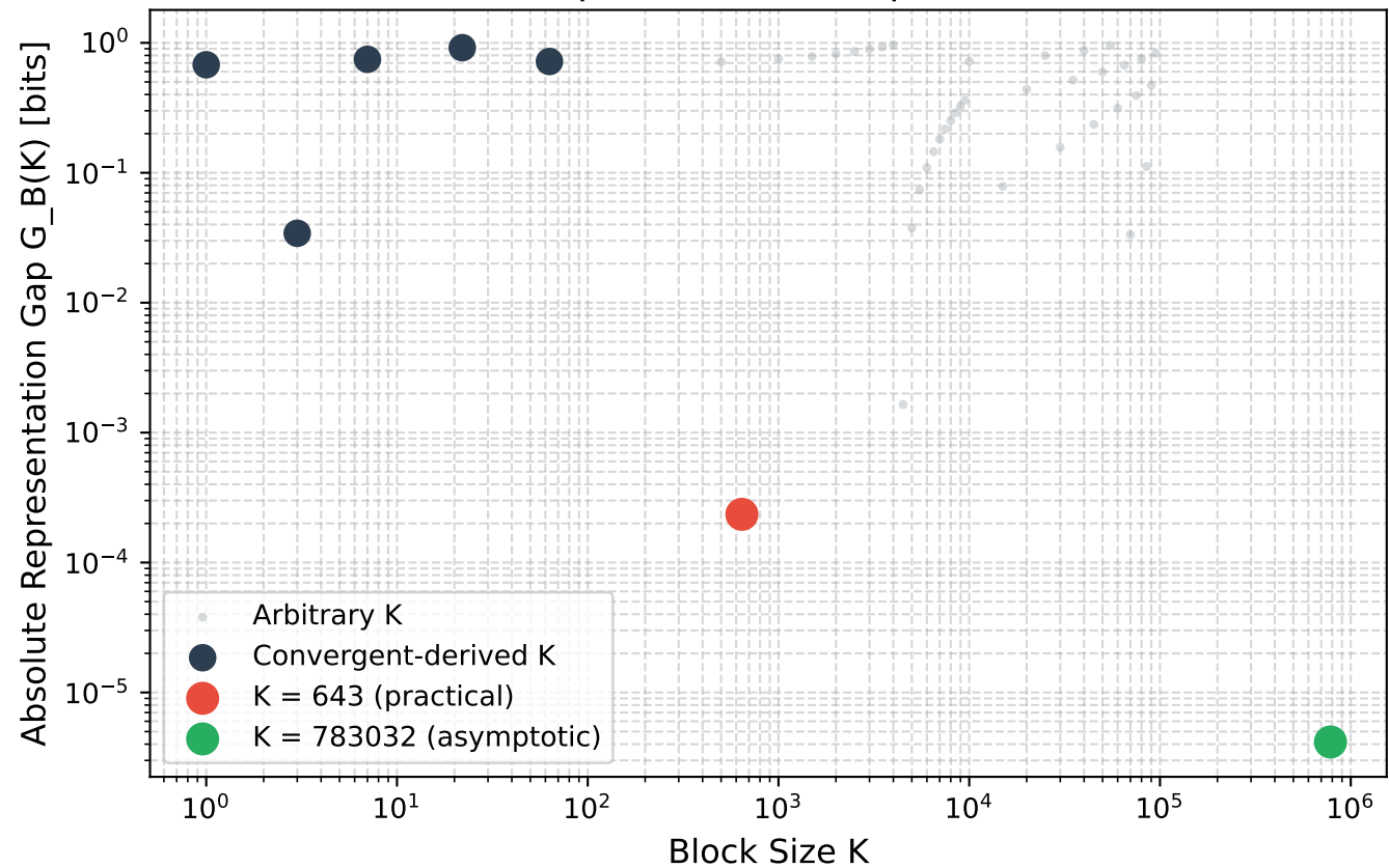
Absolute Representation Gap vs. Block Size
