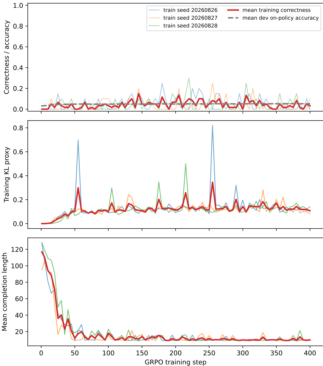
Figure 1. GRPO training trajectory
