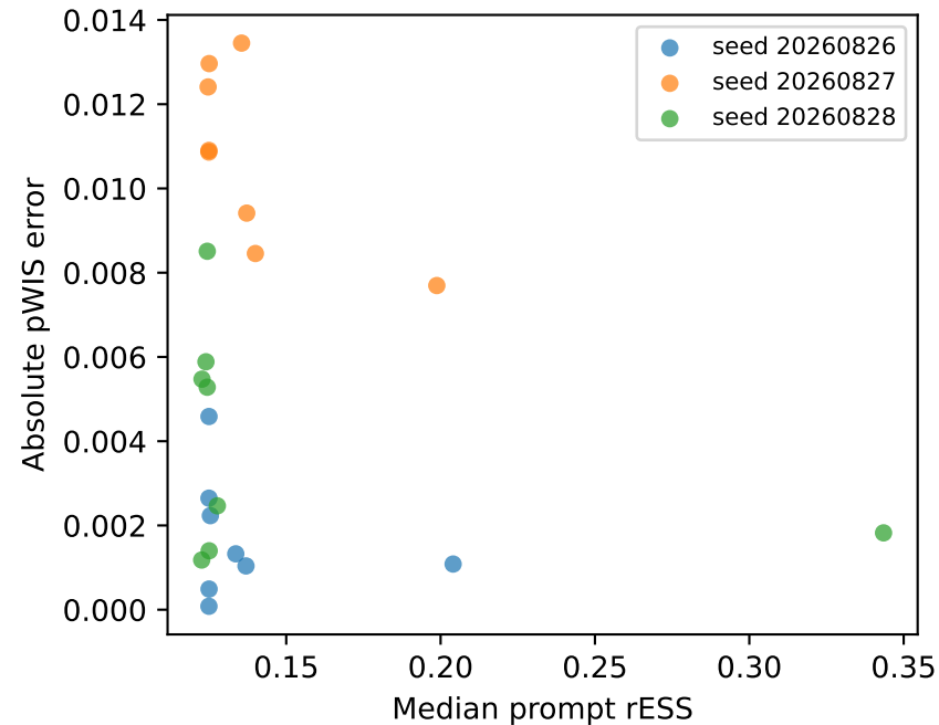
Figure 3. Offline overlap diagnostics vs OPE error (test)
