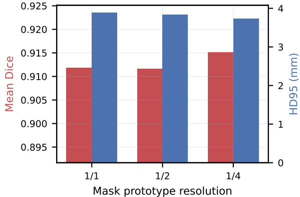
Mask head resolution
