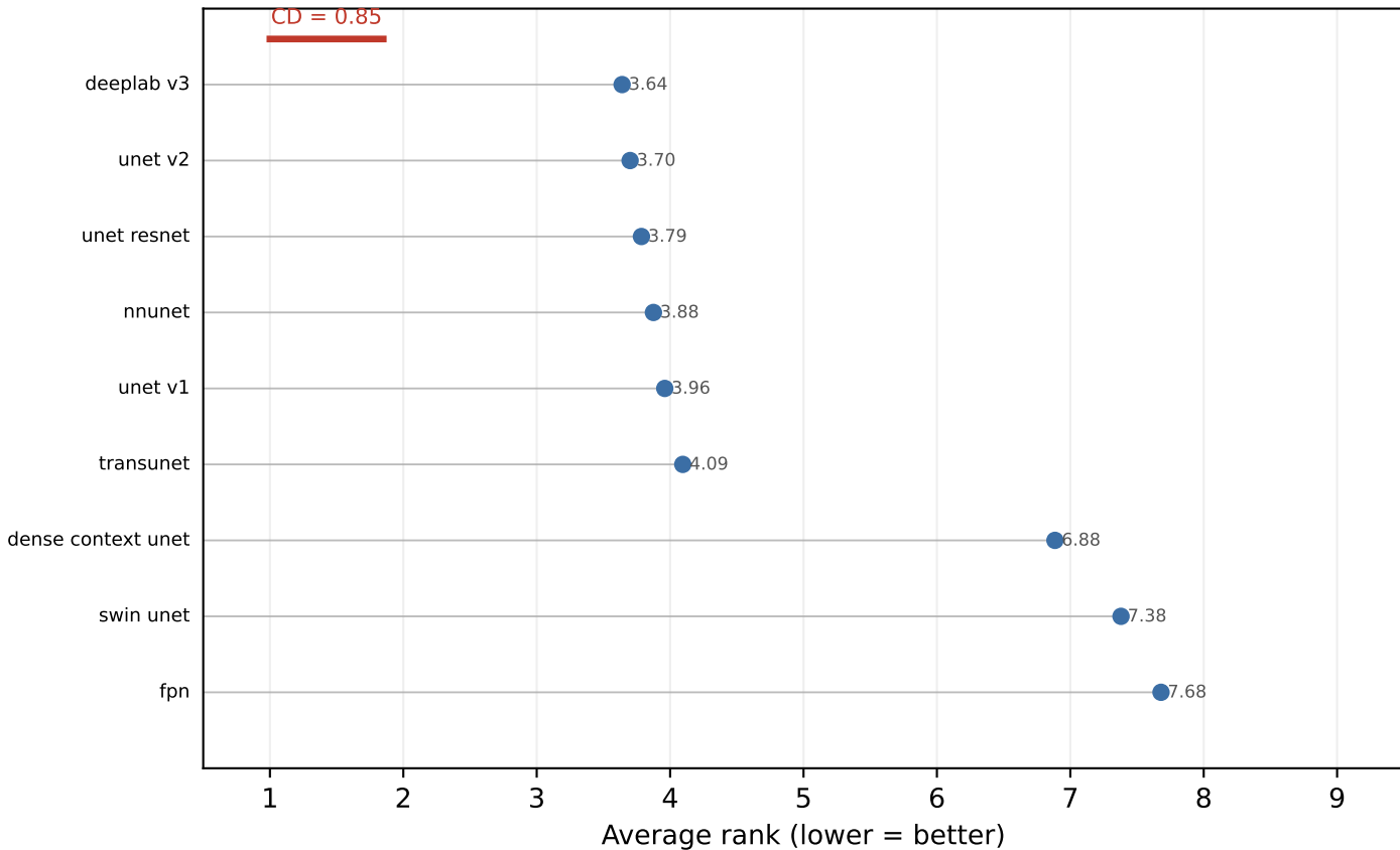
Critical-difference diagram (per-sample Dice, Nemenyi \alpha=0.05 )
