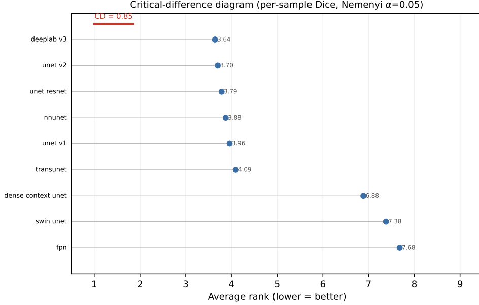
Figure 3: Critical-difference diagram (average ranks on per-sample Dice, Nemenyi test). Lower average rank is better.
