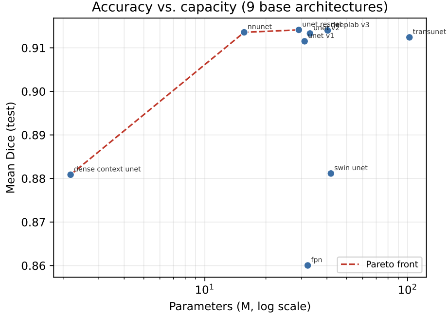
Figure 2: Accuracy–cost Pareto frontier. Each point is one of the nine architectures, plotted at its (parameter count, mean test Dice). The Pareto front is highlighted.
