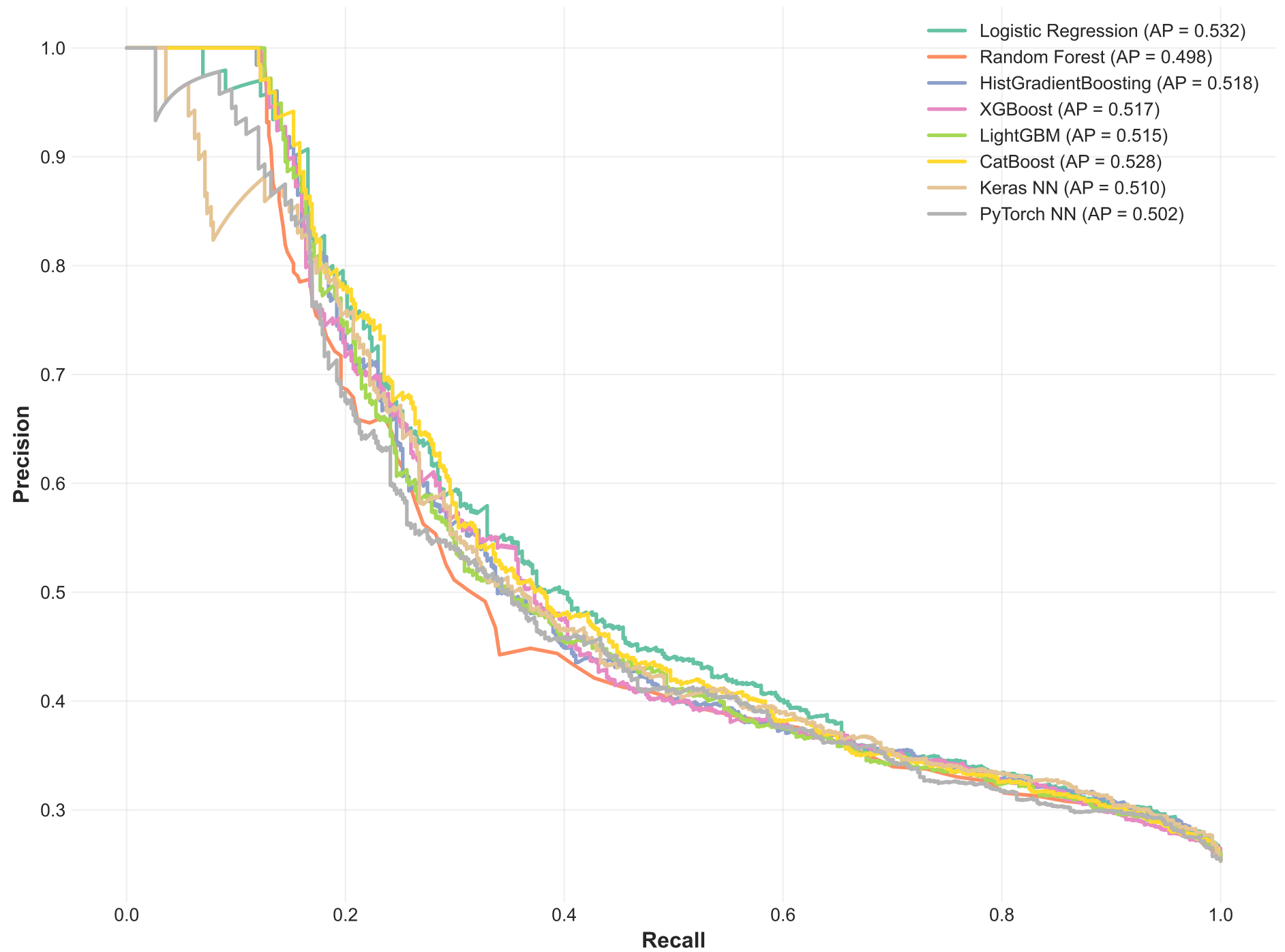
Precision-Recall Curves - Model Comparison
