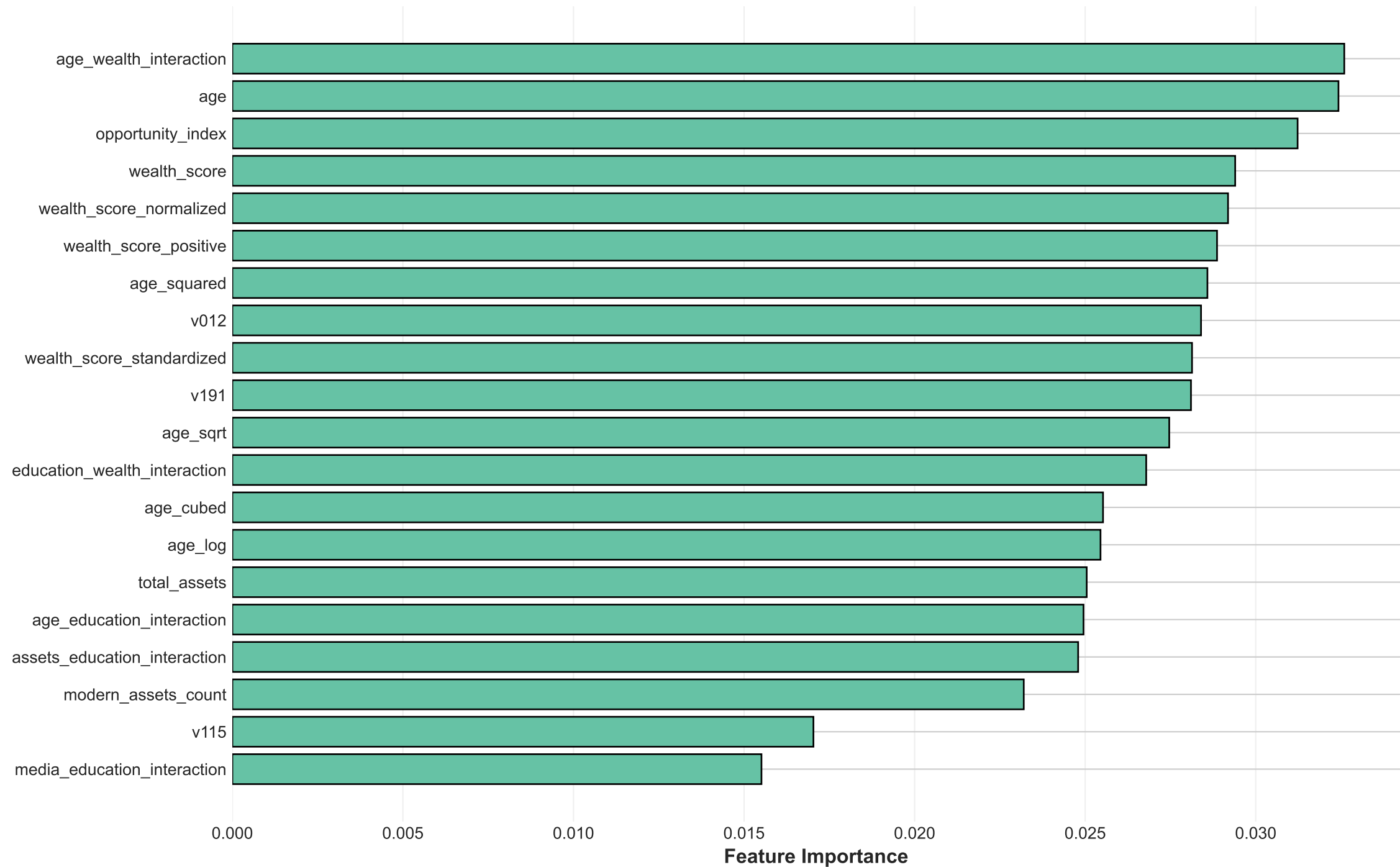
Top 20 Feature Importances (Random Forest)
