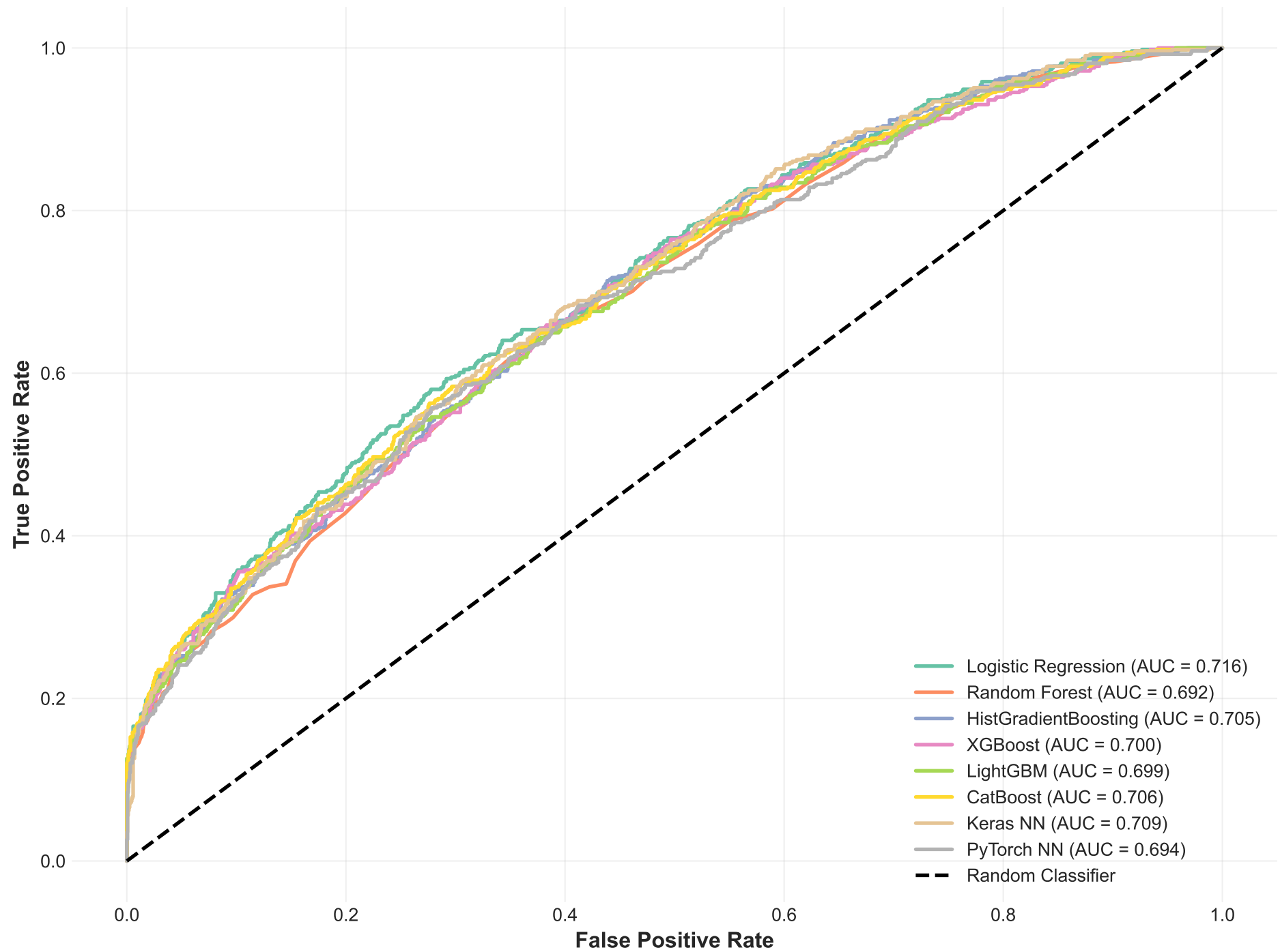
ROC Curves - Model Comparison
