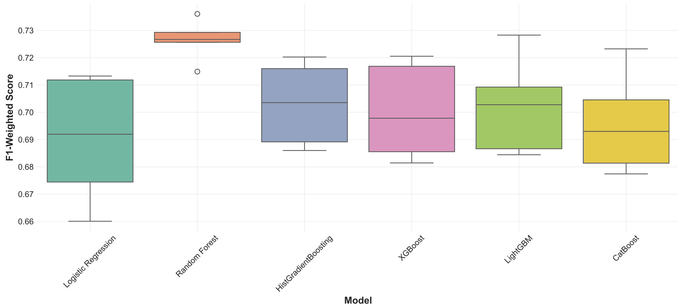
Cross-Validation F1-Weighted Scores
