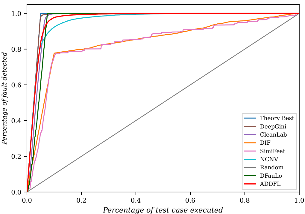
(c) Random Data Noise
