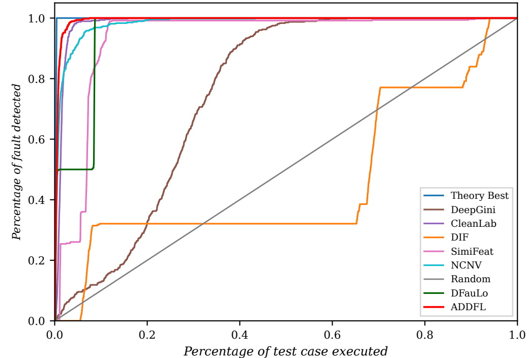
(b) Specific Label Noise
