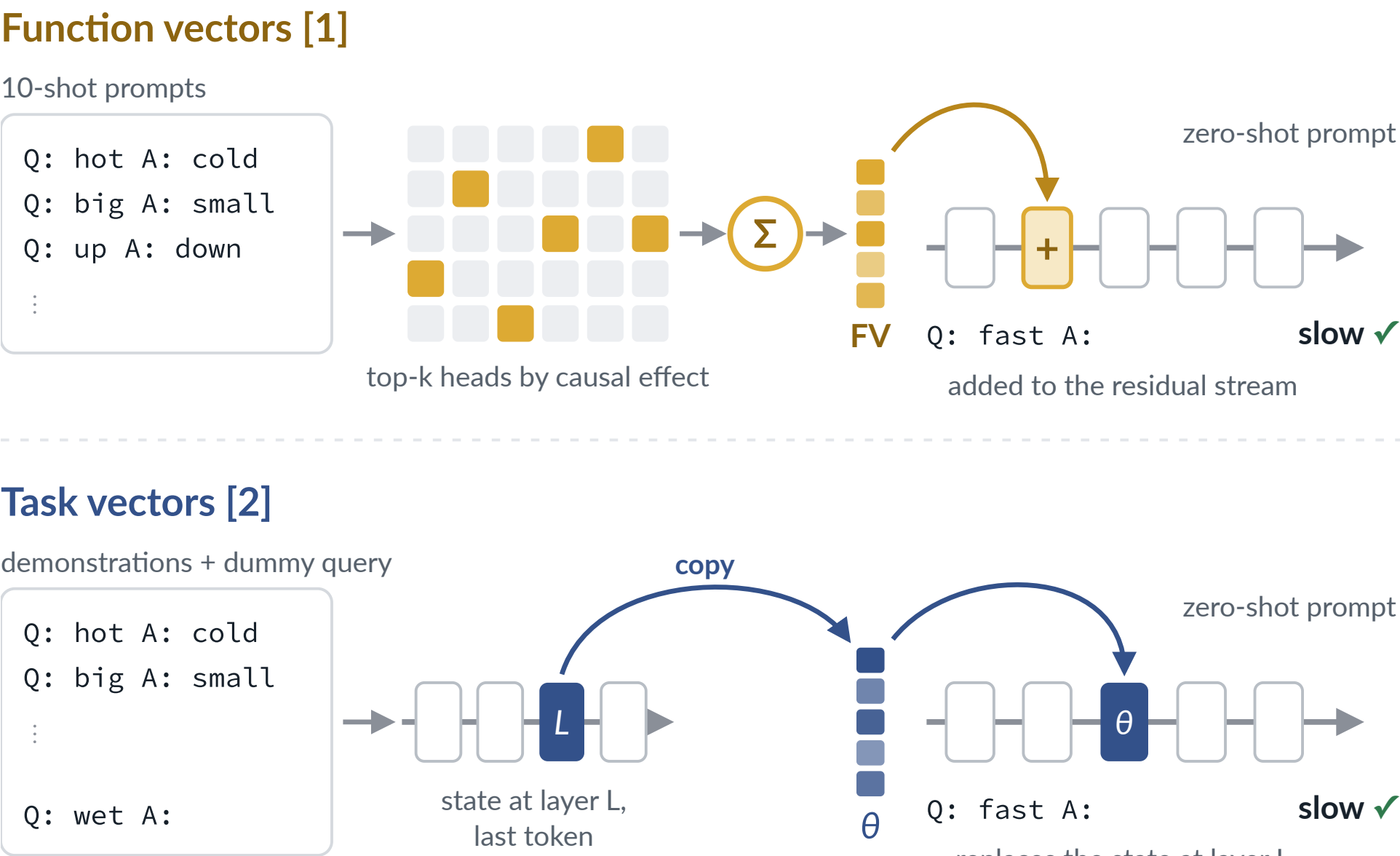
Figure 1: The two interventions, reimplemented in NNsight [3] ; the Kaggle Gemma runs use PyTorch hooks.
