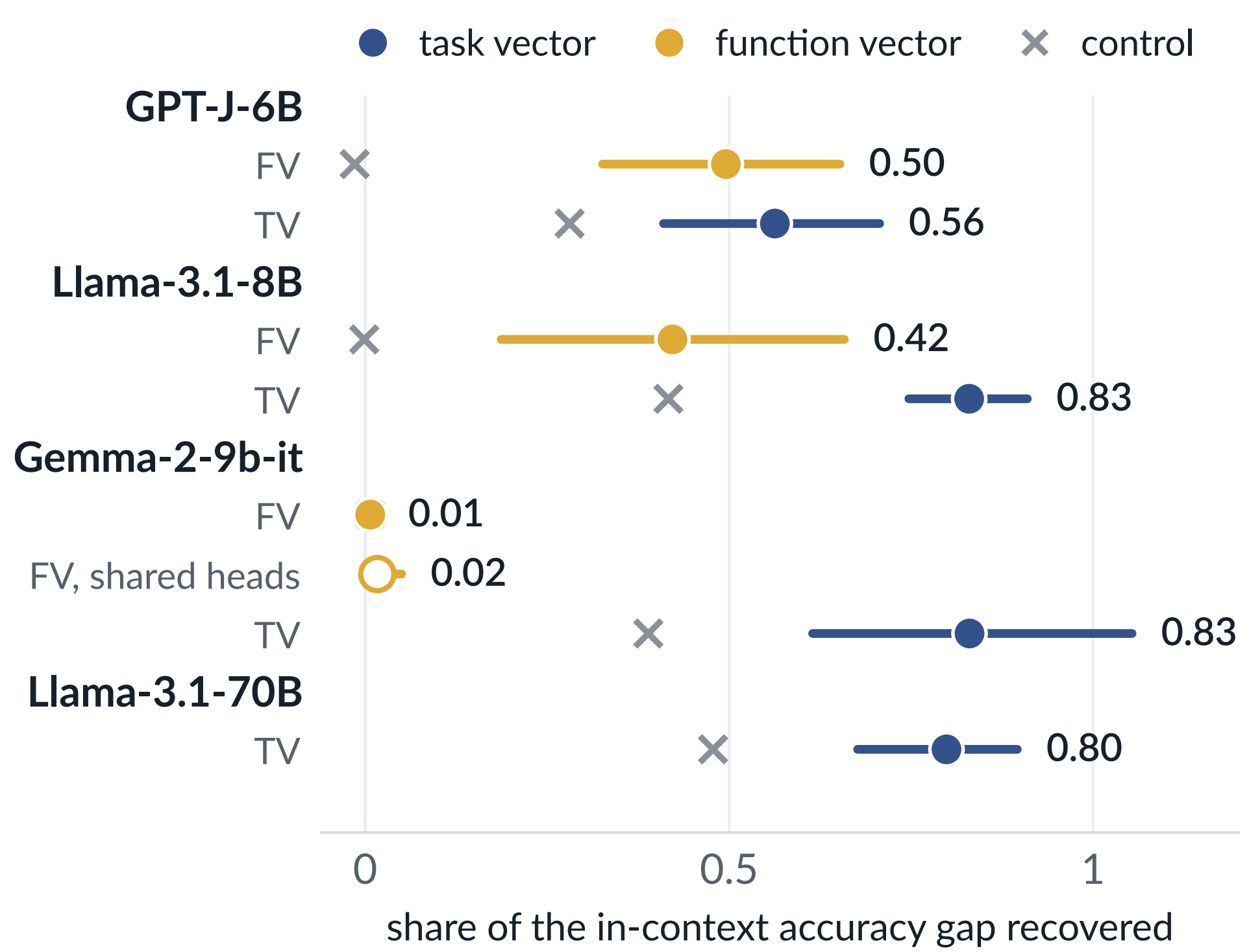
Figure 2: Best-layer recovery with task-bootstrap 95% CIs; × marks the control. Choosing the layer on the scored data favours the real vector.
