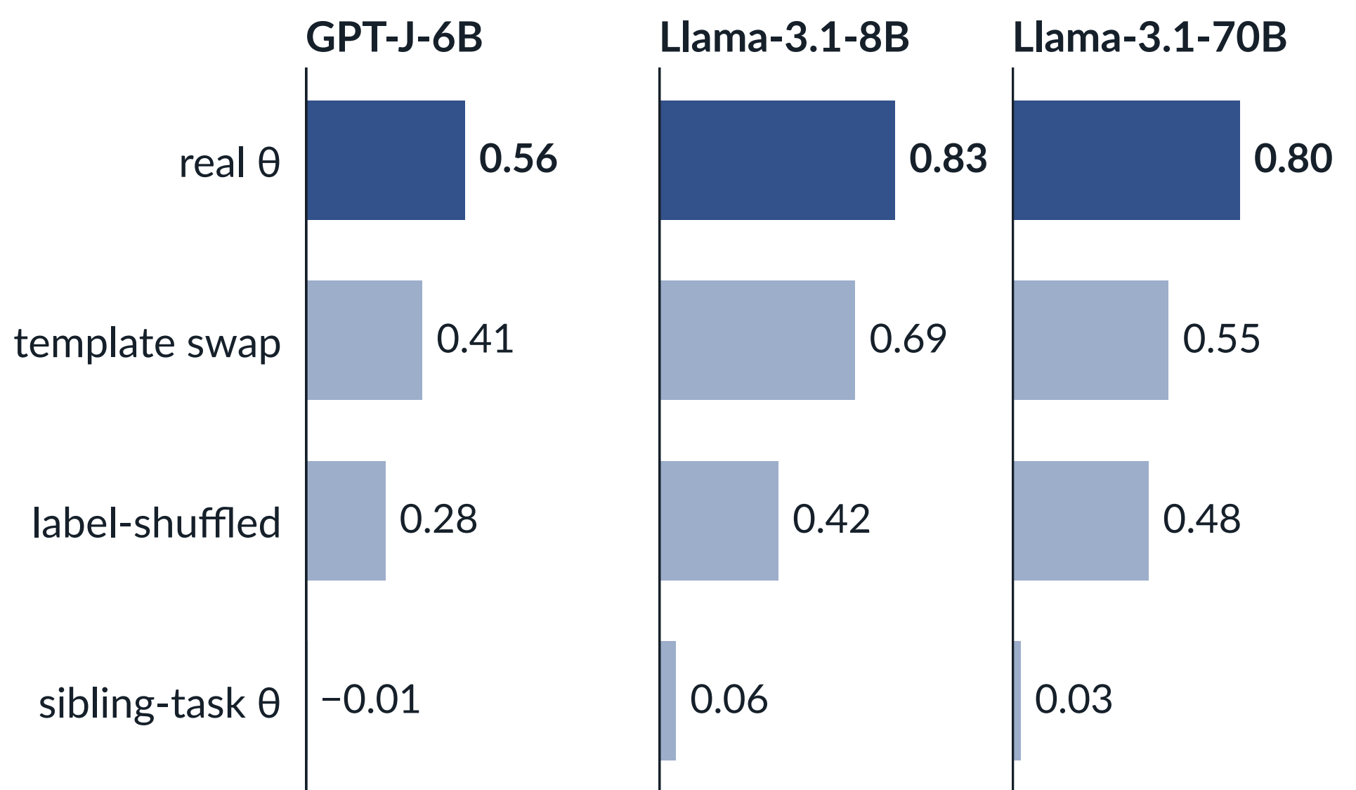
Figure 6: Exploratory recovery at the real TV's layer.
