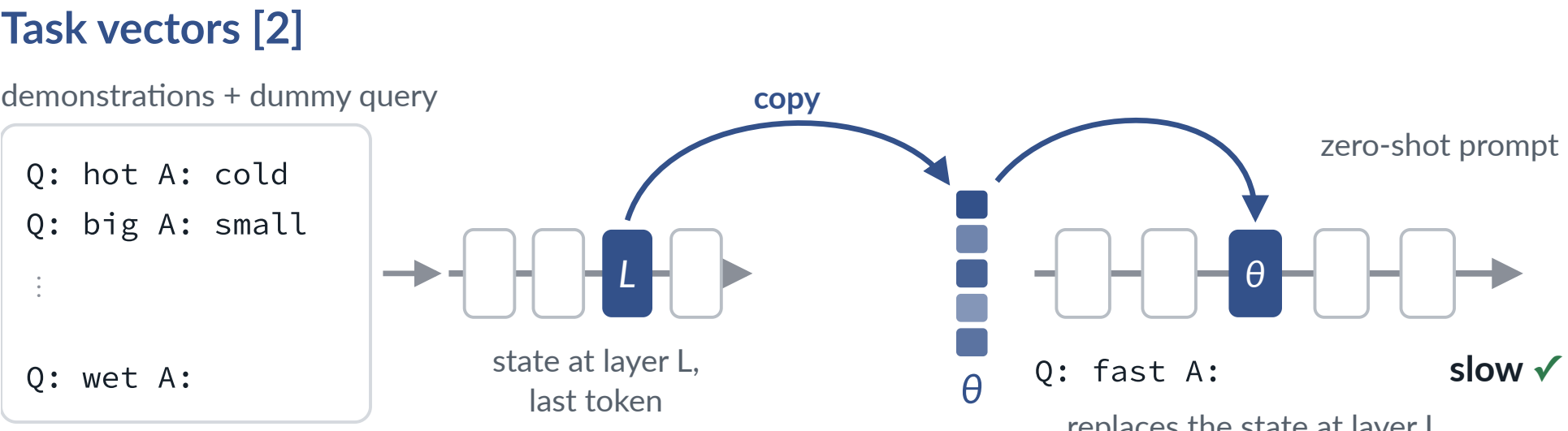
Figure 1: The two interventions, reimplemented in NNsight [3] ; the Kaggle Gemma runs use PyTorch hooks.
