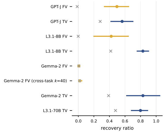
Figure 1: Method recovery estimates with task-clustered 95% CIs (bars) and matched controls (x). The hollow marker is the Gemma-2 FV arm rebuilt with Todd et al.’s cross-task head selection at k = 40 .
