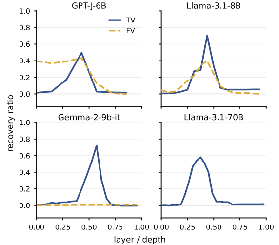
Figure 2: Recovery by layer depth. FV is dashed; TV is solid.
