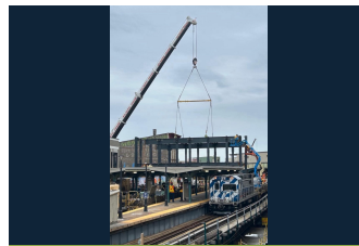
MYRTLE AVENUE STATION - PLATFORM OVERPASS
