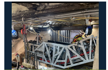
GRAND CENTRAL STATION ADA UPGRADES - ESCALATOR
