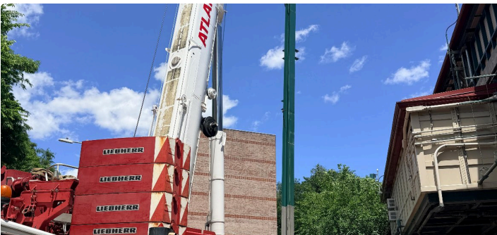
MIDDLETOWN ROAD STATION — ADA UPGRADES, ELEVATOR INSTALLATION
