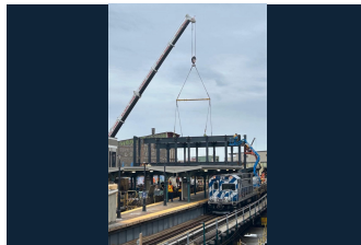
STEEL ERECTION - ACTIVE STATION
