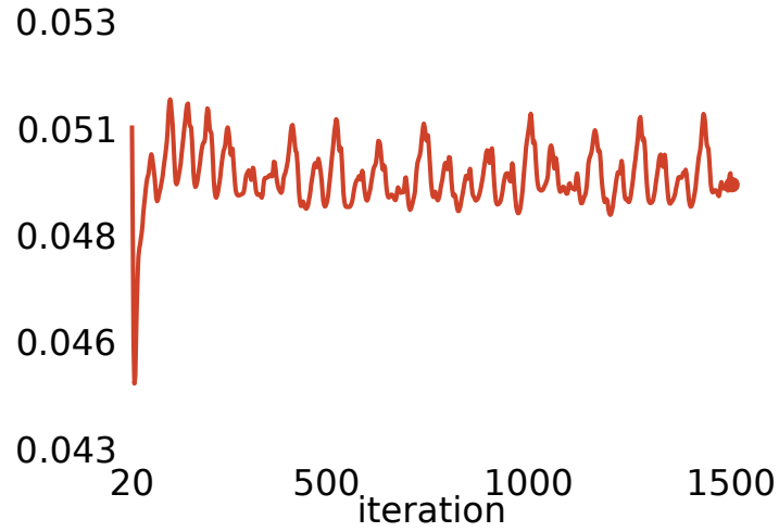
Fig. 14. Drag-coefficient history; C_D averages at around 0.0494 (shown from iteration 20).
