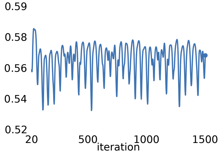
Fig. 13. Lift-coefficient history; C_L averages at around 0.567 (shown from iteration 20).
