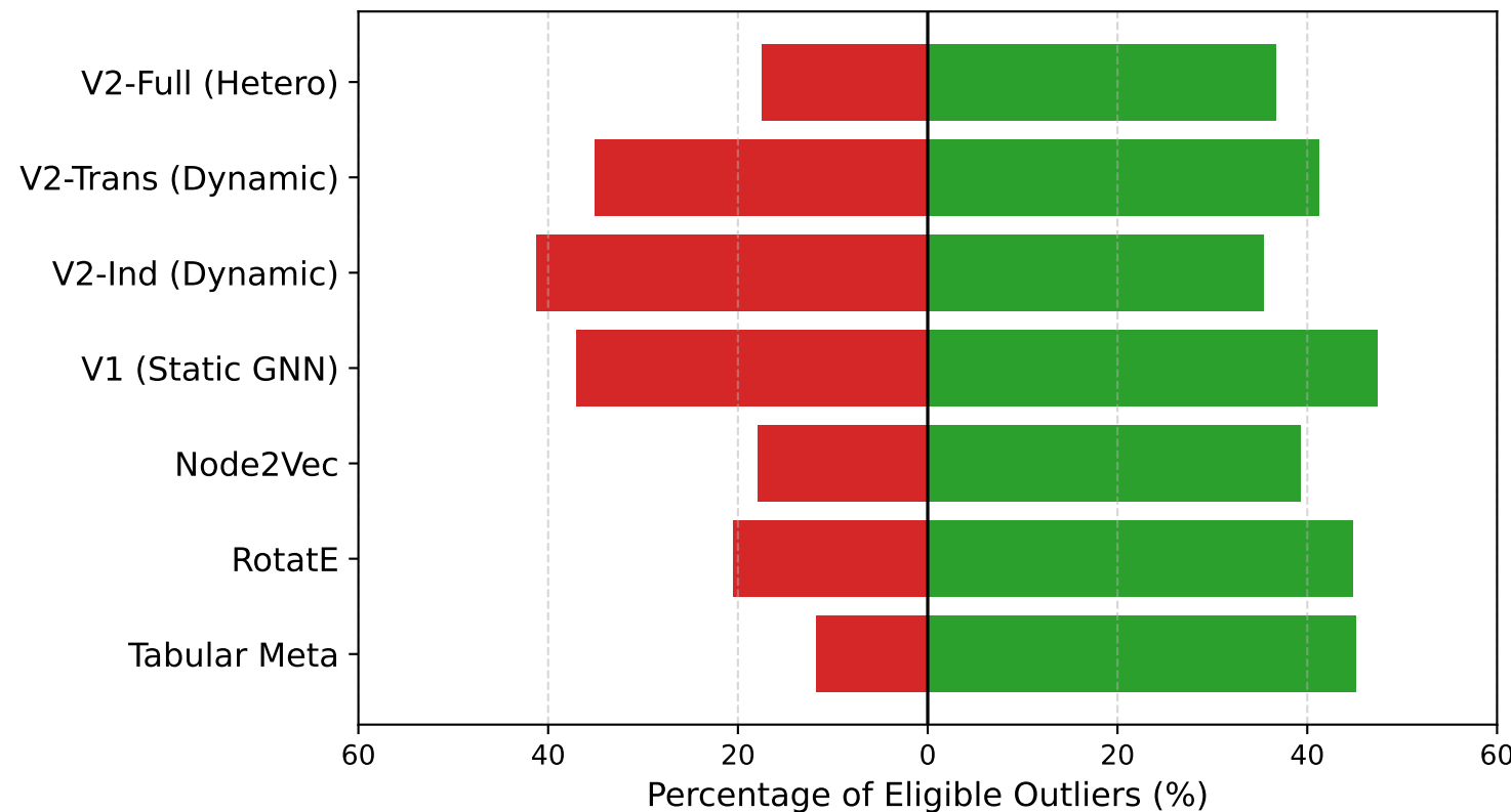
(a) vs. Weak Baseline (Stats + Time)
