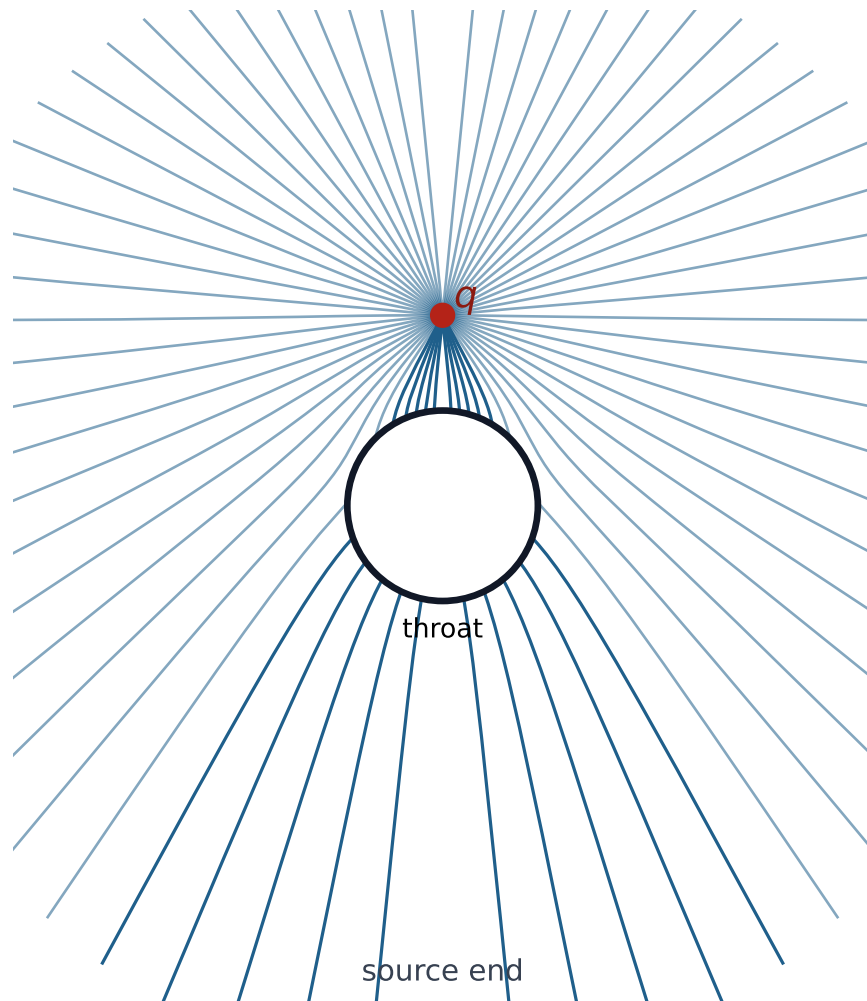
Flat thin-shell wormhole: zero Wheeler-flux field lines
