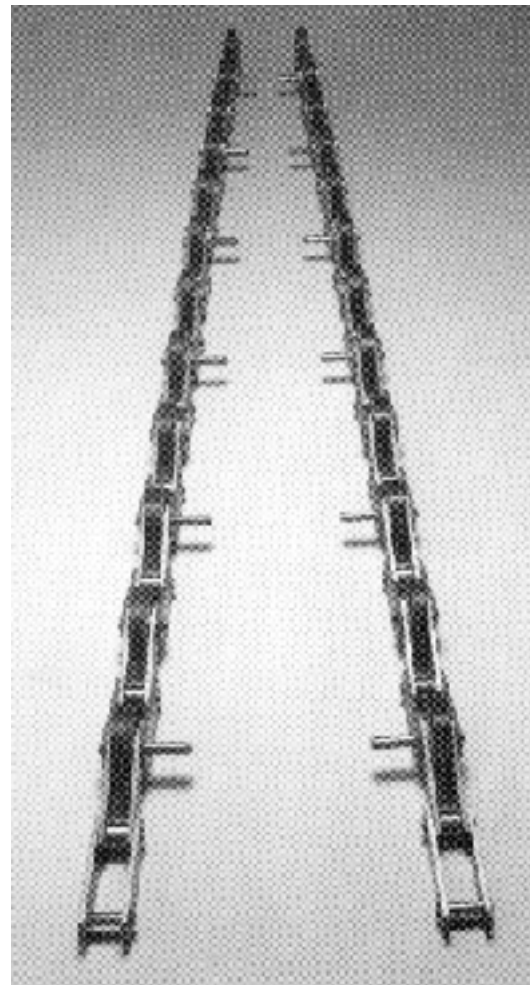
Step Chain, 1 pair assembled with (24) A42860 M-P12963 rollers between the links.
