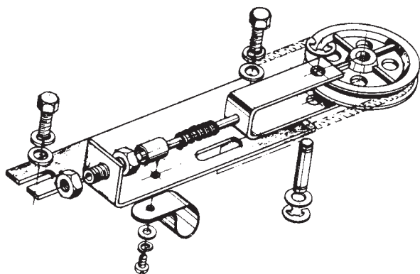
Tension pulley assembly, RH HH-3-6RH
