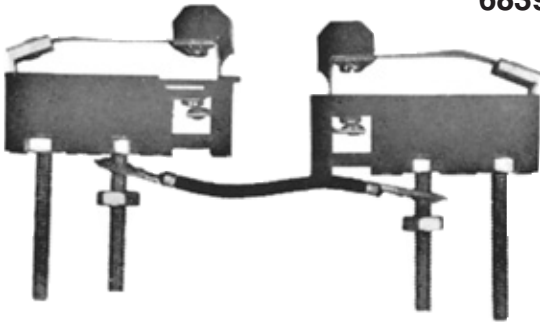
Brush switch. Double unit with fiber cams and connecting shunt.
