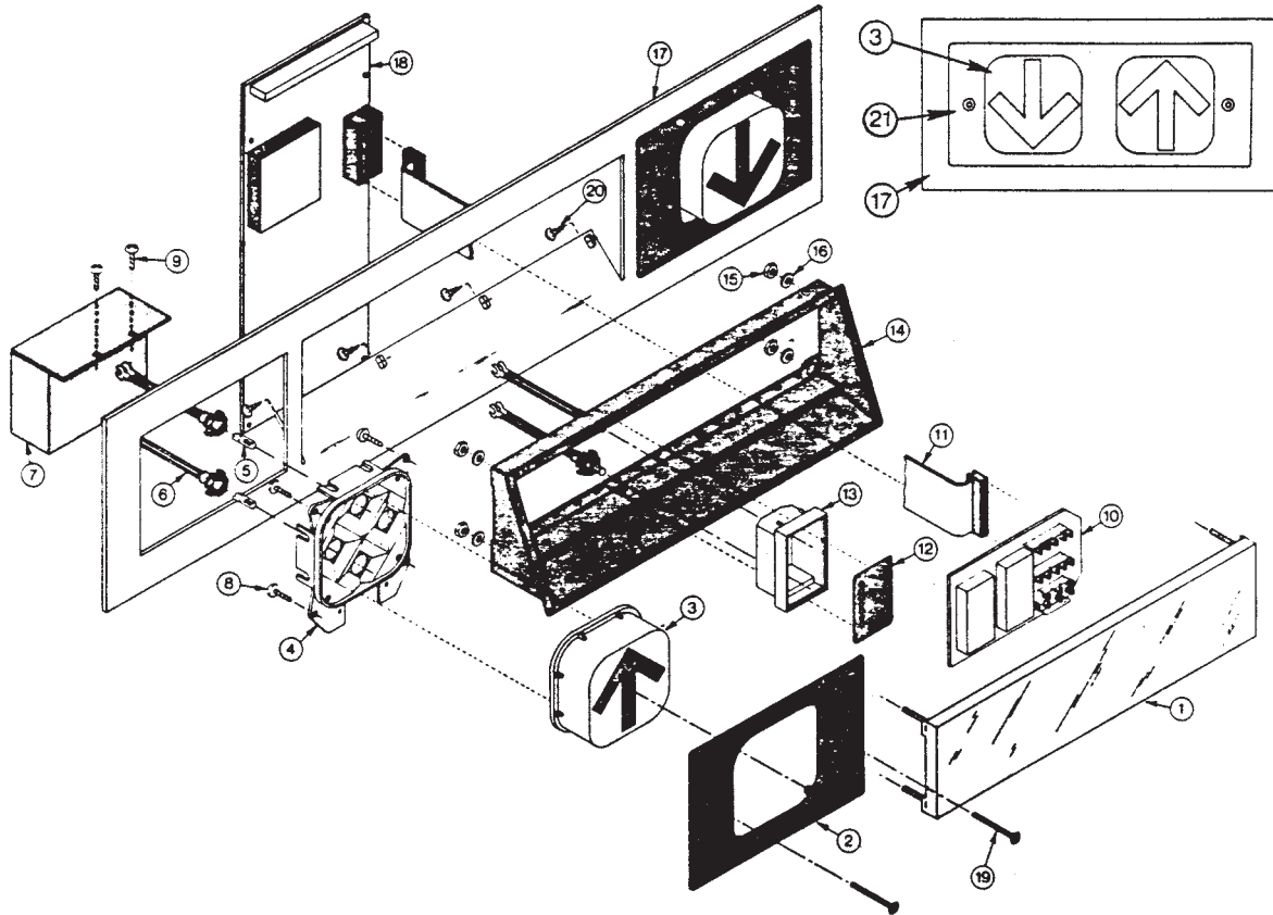
HALL LANTERN AND P.I. (TYPICAL ASSEMBLY)
