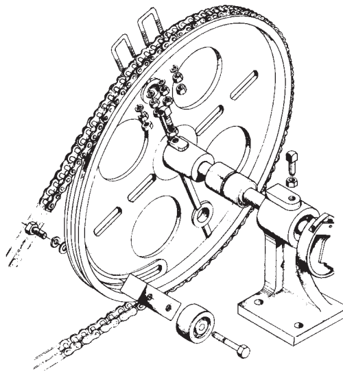
MOD operator drive pulley and bearing block assembly, RH OP-10-5RH
