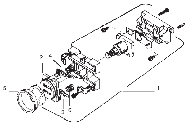
Type "A" Car Switch Assembly
