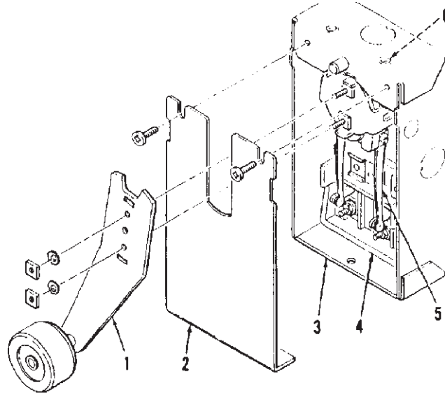
A6098B3 LIMIT SWITCH - Single Pole, Single Throw - Breaking as shown.
