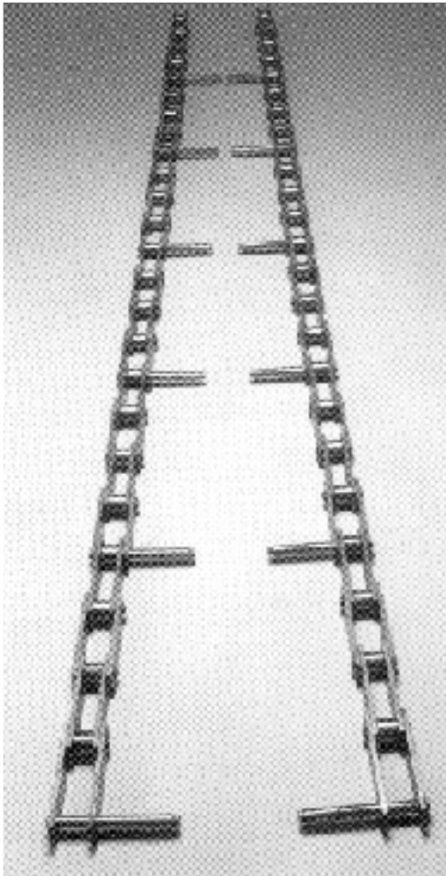
Step chain, 1 pair assembled with (24) 35671 M-P12963 rollers between the links.
