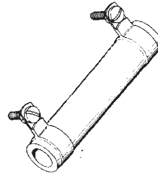
30 WATT RESISTOR - Lava tube 10-1/8" long with adjustable band and conductor.
