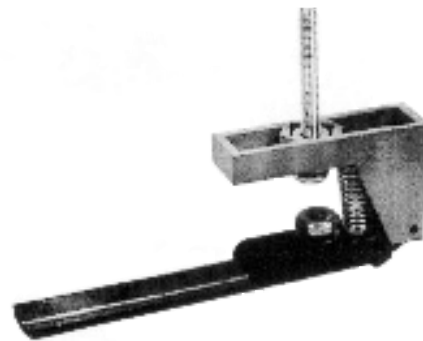
Position indicator brush, selector insulated butt. Print number; 129038. 9729045
