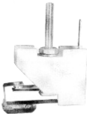
Selector brush switch, long. Print number; 102336. 9823360
