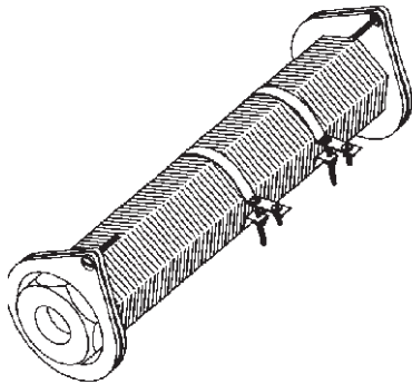
700 WATT RESISTOR - Lava tube 10-1/8" long with adjustable band and conductor.
