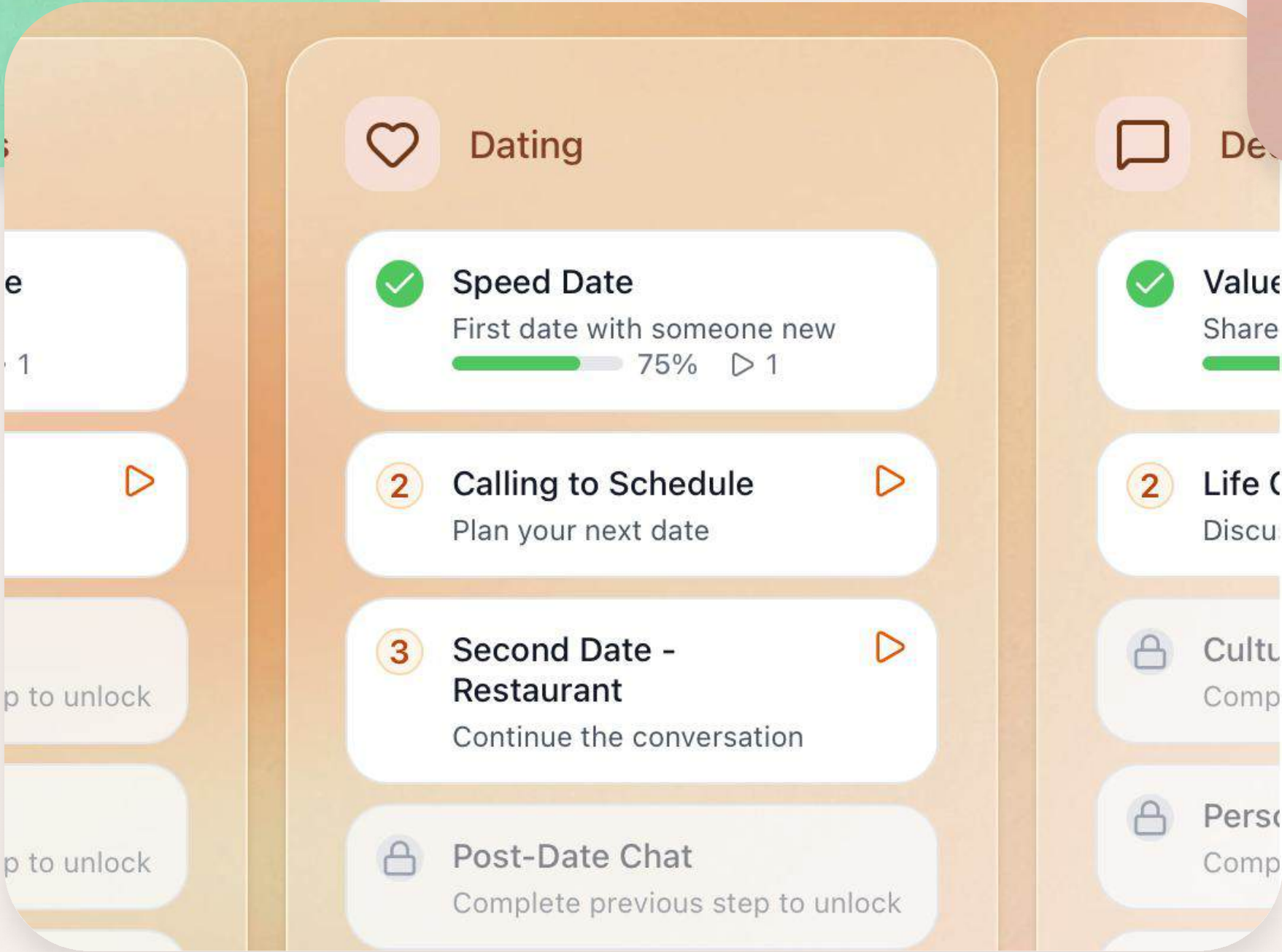
Multi-step scenarios
