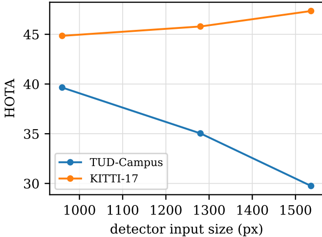
Figure 3. Input-size sweep on the two dense clips. Resolution changes the detection set rather than gating it, so its effect is sequence-dependent: it hurts on TUD-Campus and helps on KITTI-17.
