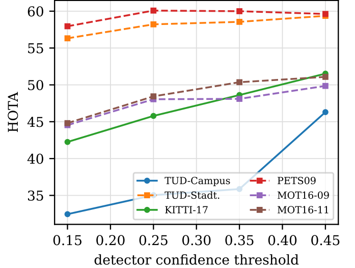
Figure 1. HOTA vs. detector confidence threshold per video. Raising the gate from the lowest to the highest threshold never net-lowers HOTA on any clip; the climb is steepest on the dense, low-precision clips (solid lines).
