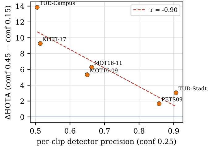
Figure 2. The HOTA gained by raising the gate (conf 0.45 minus conf 0.15) against per-clip detector precision. Low-precision clips gain most ( r = -0.90 ).
