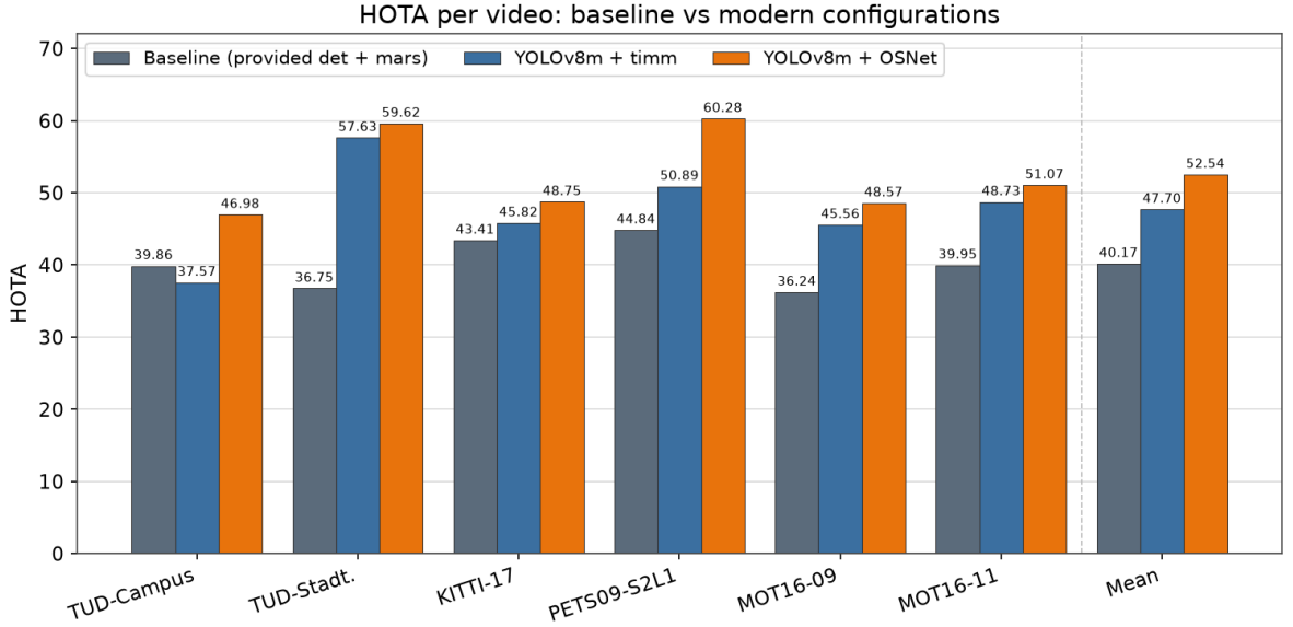
Figure 4: Per-video HOTA for the baseline and the two modern configurations.
