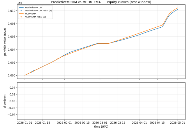
Fig. 2. Cumulative equity curves over the 4-month test window (Jan – Apr 2026). The two strategies track each other almost perfectly: PredictiveMCDM (forecast-driven) net APY 3.36% versus MCDMEMA (reactive) 3.44%. The gap is 8 bp; on this window the forecast pays its overhead but does not earn it back. Section VI decomposes which layer of the transfer hypothesis is responsible.
