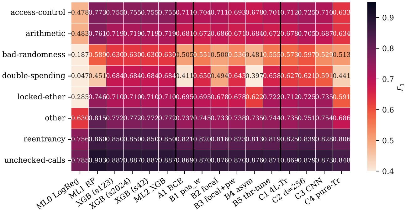
Per-class F_1 : classical ML (left) vs.\ Conv-Transformer 10-config ablation (right)
