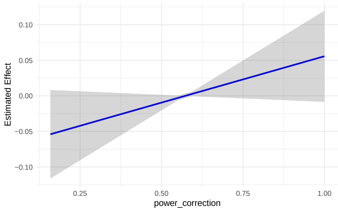
Estimated effect for power_correction
