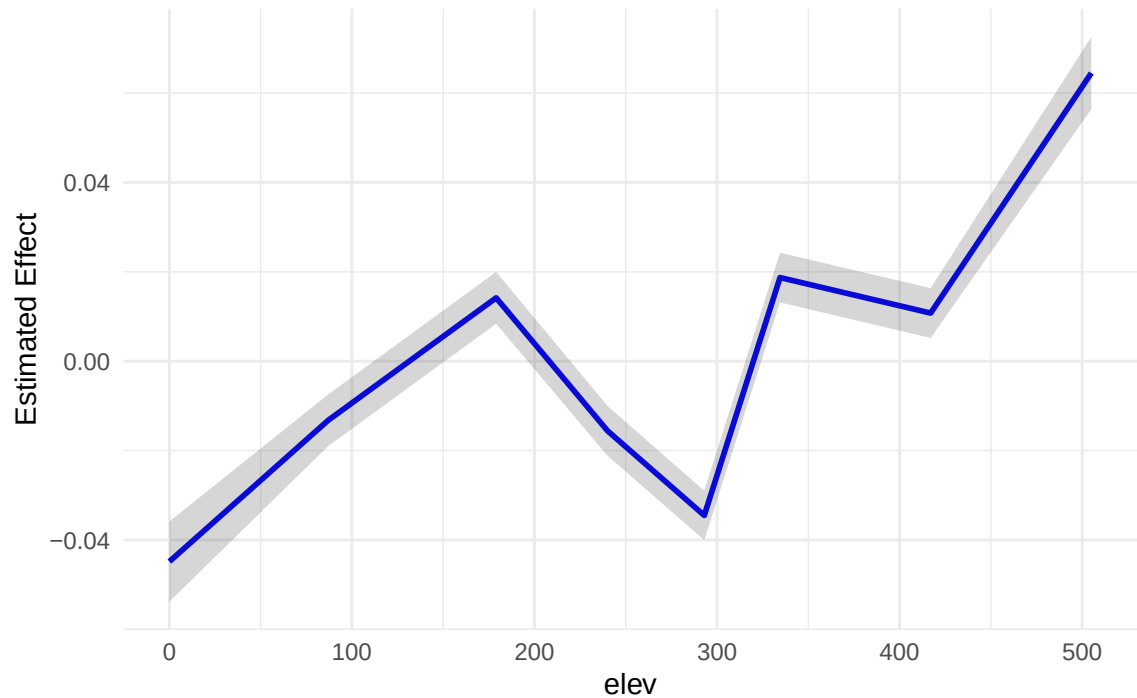
Estimated effect for elev
