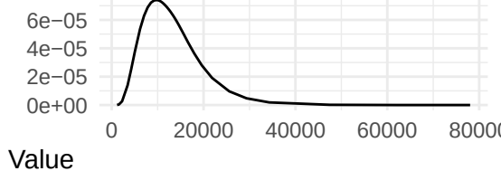
Precision for wind
