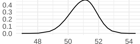
Precision for the Gaussian observations
