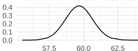
Precision for the Gaussian observations
