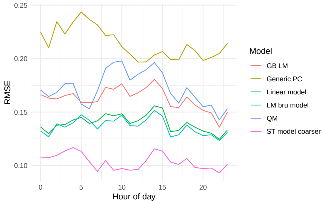
Model performance by hour of day
