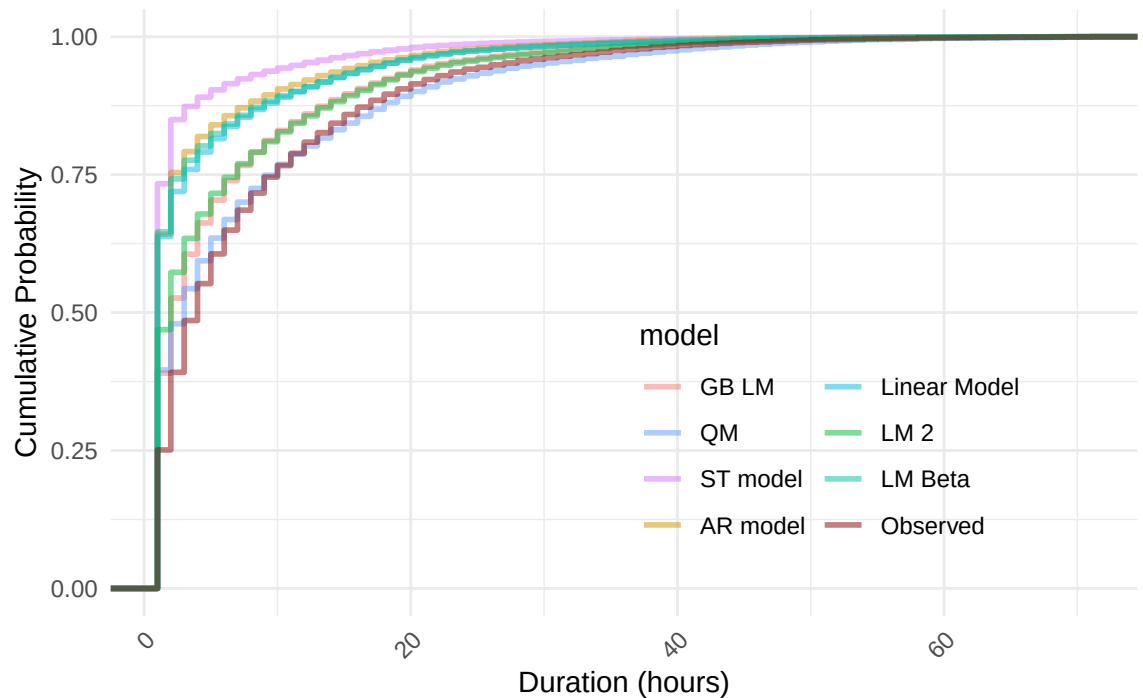
Cumulative Distribution of Low Wind Events Duration
