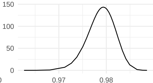
Rho for u
