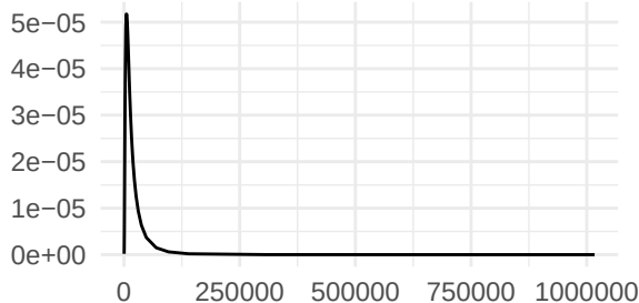
Precision for wind
