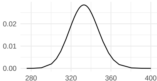
Precision for the Gaussian observations
