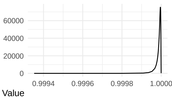
Rho for u
