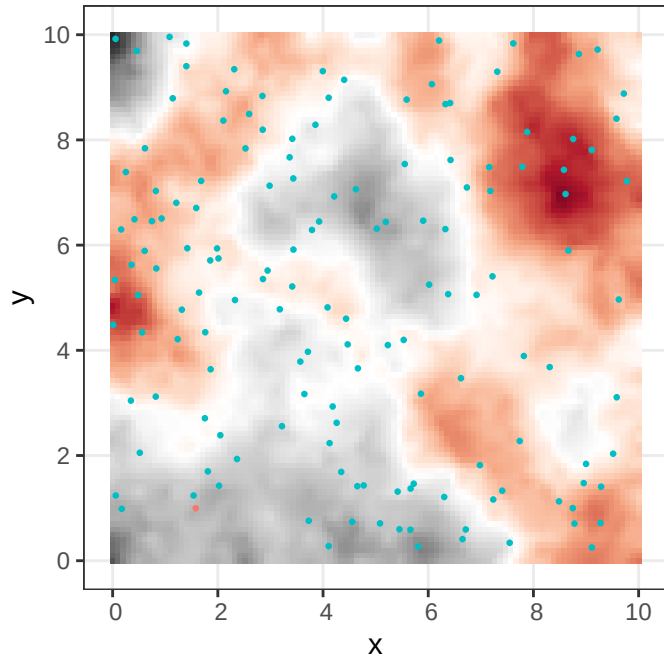
True field
