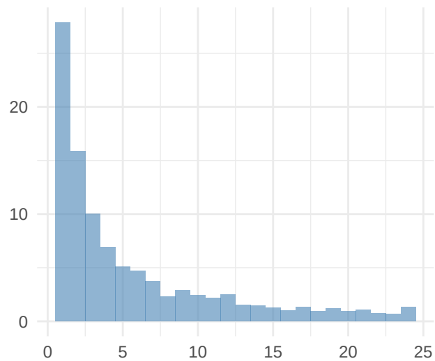
Observed
