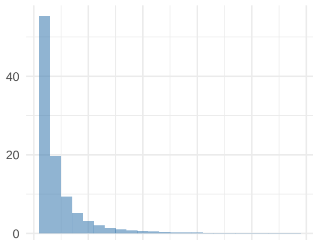
AR2 model
