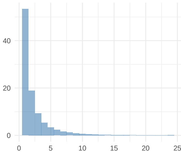
Spatio-temporal model coarse
