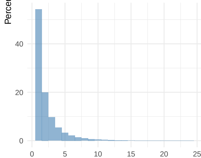
1D SPDE model
