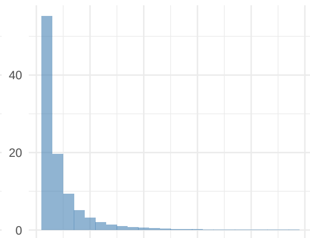
AR2 model
