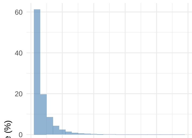
AR1 model
