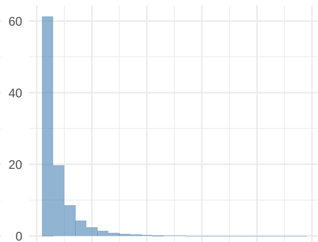
AR2 model
