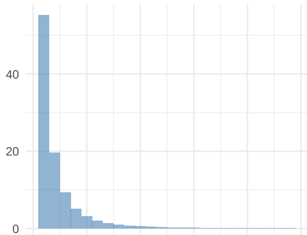
AR2 model
