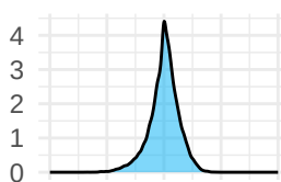
AR1 model
