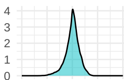
LM+hour model
