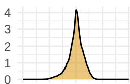
Linear model
