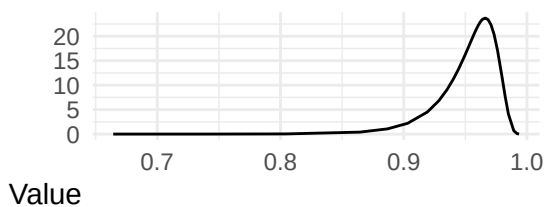
Rho for u
