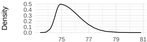
Precision for the Gaussian observations
