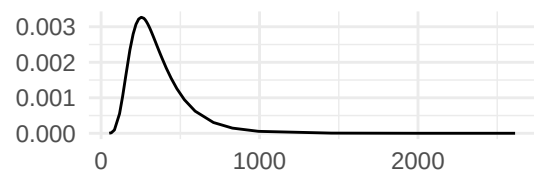
Precision for u
