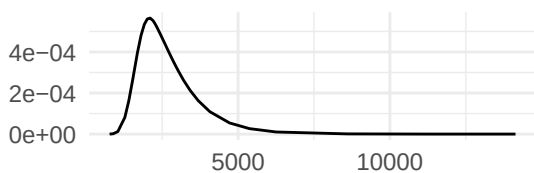
Precision for wind
