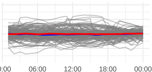
Spatio-temporal model
