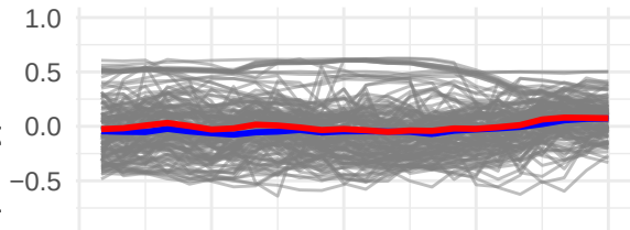
Linear model
