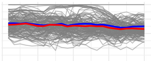
Generic PC
