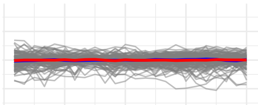
Spatio-temporal model
