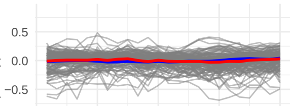
Linear model
