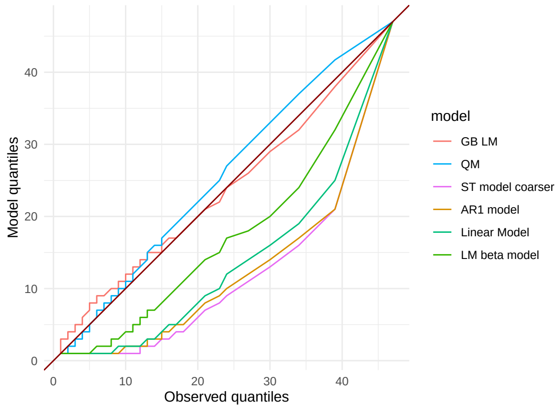
Q-Q Plot of Low Wind Event Durations
