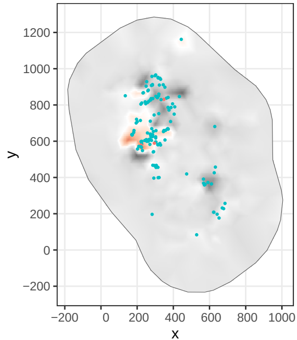
Post. mean
