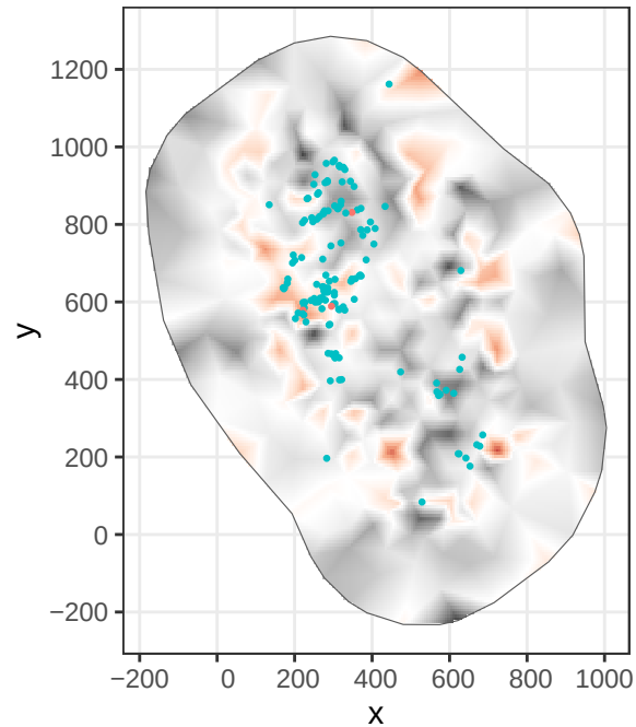
Post. sample
